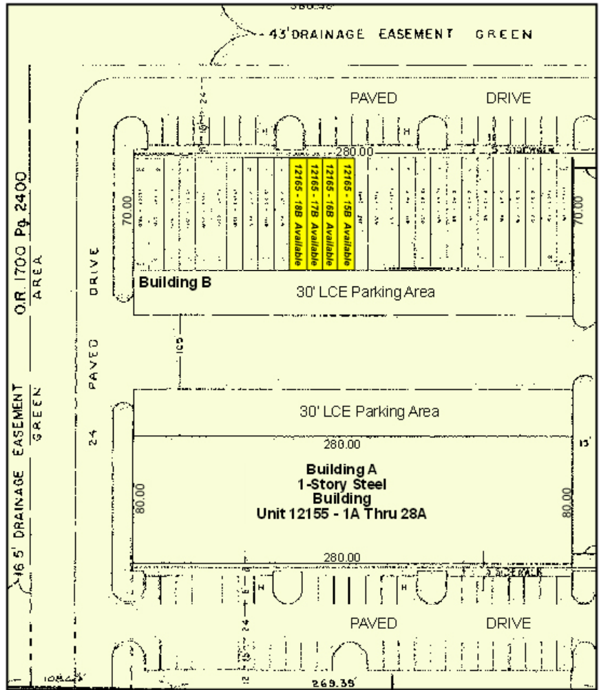
Site Plan
